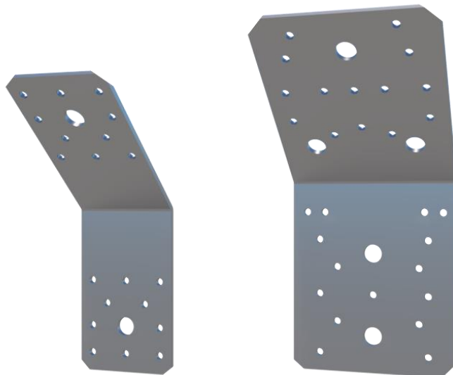
AB 135° 90 Cod. 390201090652
